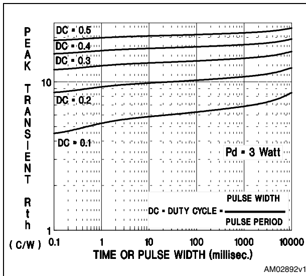
Figure 14. PowerSO-20: with external heatsink
