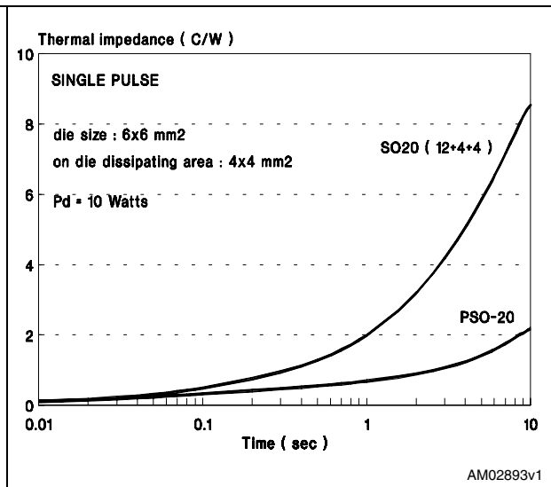
Figure 15. Thermal impedance of PowerSO-20 and standard SO20
