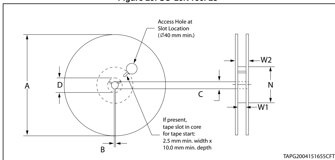
Figure 29. SO-16N reel 13"
