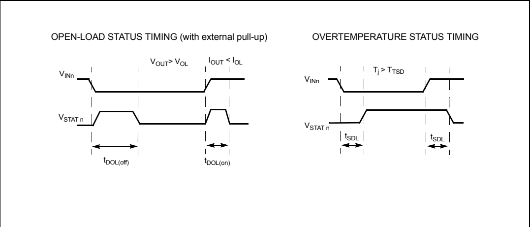
Figure 4. Status timing
