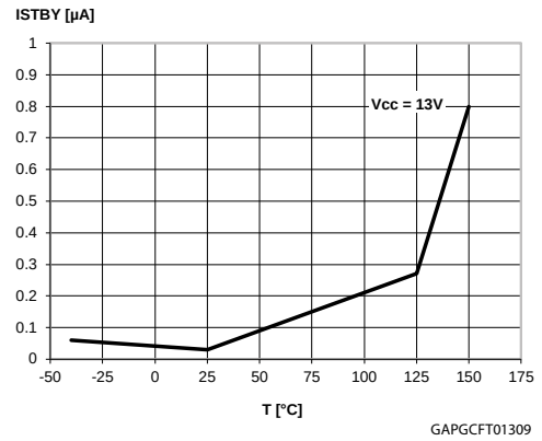
Figure 16: Standby current
