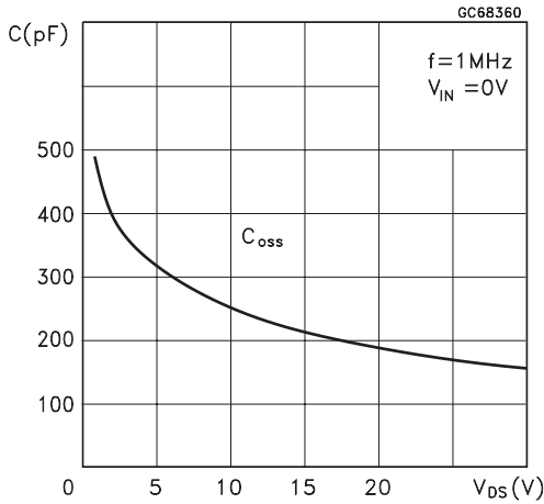
Figure 12. Capacitance Variations
