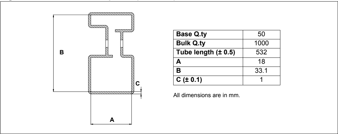
Figure 29. P 2 PAK tube shipment (no suffix)
