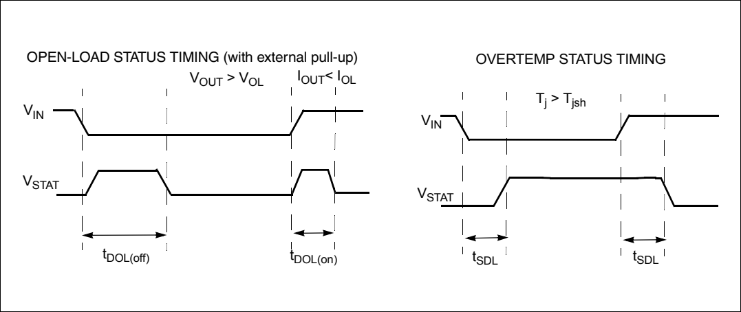
Figure 4. Status timings
