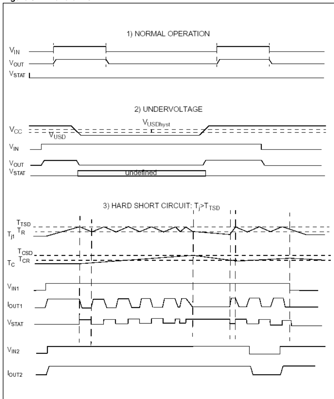
Figure 8. Waveforms
