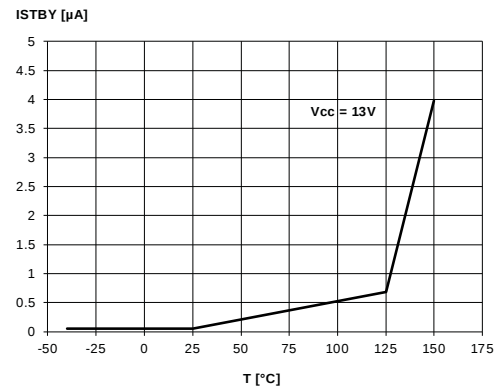
Figure 9: Standby current
