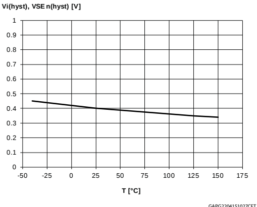
Figure 15: Logic Input hysteresis voltage
