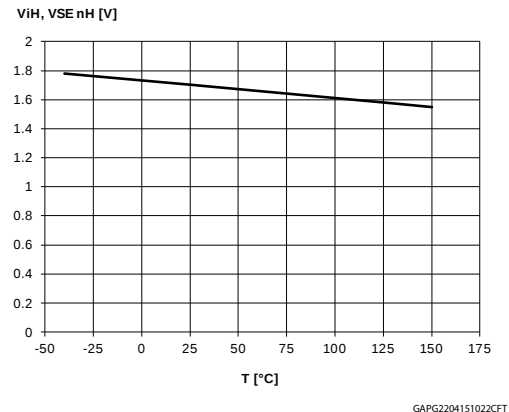
Figure 11: Logic Input high level voltage
