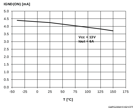
Figure 10: IGND(ON) vs Tcase
