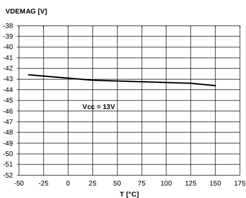
Figure 24: Turn-off output voltage clamp
