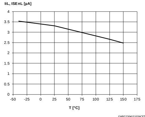
Figure 14: Low level logic input current
