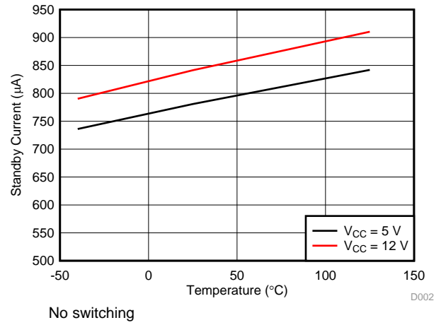
Figure 3. Standby Current ( I_{CC(ON)} ) vs Temperature
