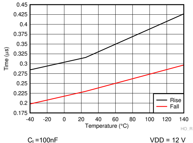
Figure 6-21. HO Rise &amp; Fall Time
