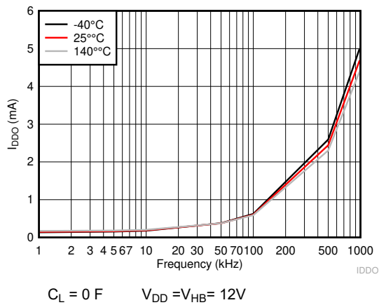
Figure 6-4. VDD Operating Current
