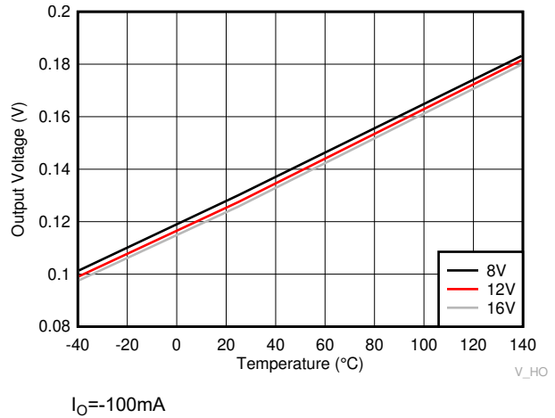
Figure 6-15. HO High Output Voltage ( V_{HOH} )
