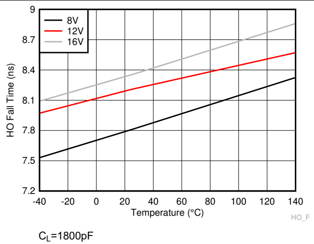
Figure 6-19. HO Fall Time
