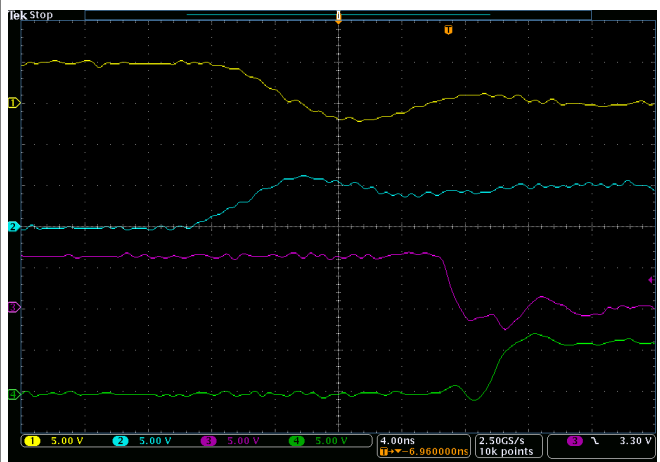
Figure 8-8. Propagation Delay and Delay Matching
