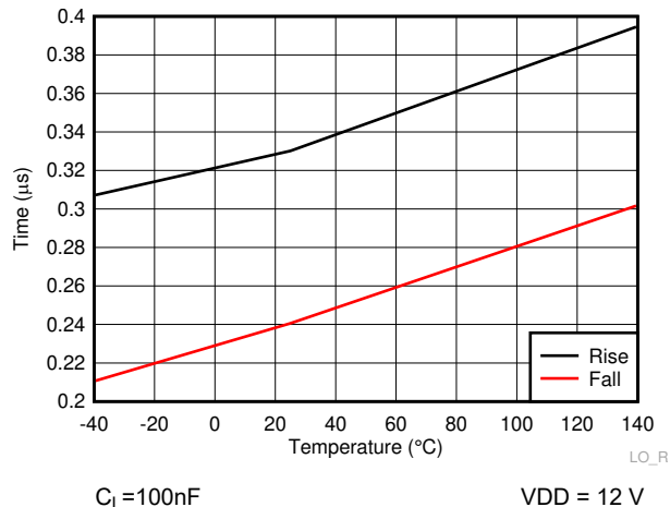
Figure 6-20. LO Rise &amp; Fall Time
