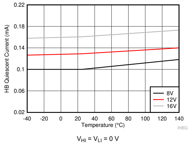
Figure 6-3. HB Quiescent Current
