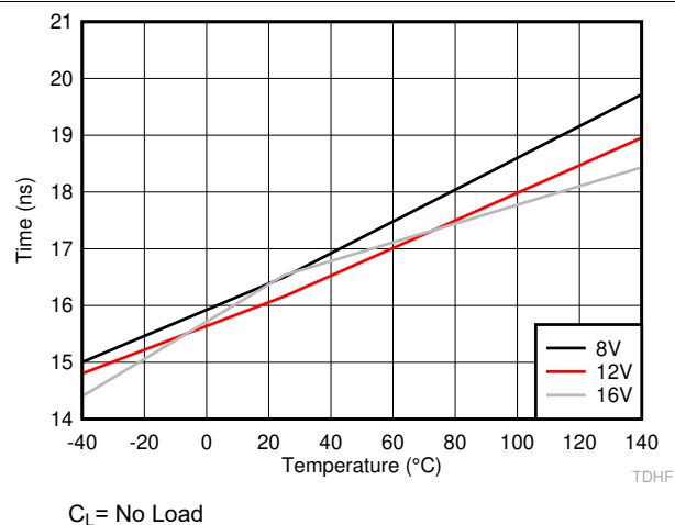
Figure 6-23. HO Falling Propagation Delay (TDHFF)
