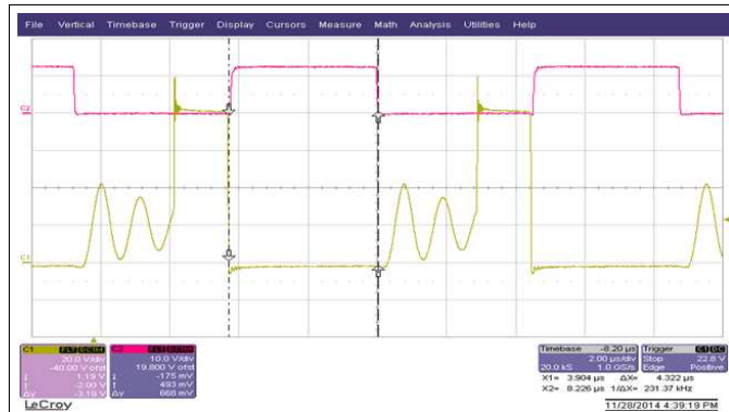
Figure 25. DRV Timing at 230 V AC , 65 W
