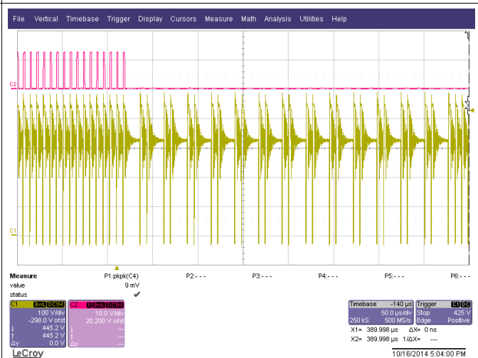
Figure 26. DRV Timing at 115 V AC , 65 W
