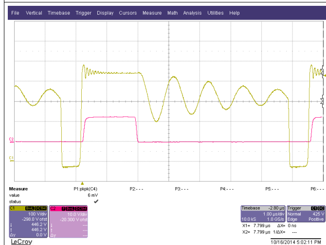
Figure 25. DRV Timing at 230 V AC , 65 W
