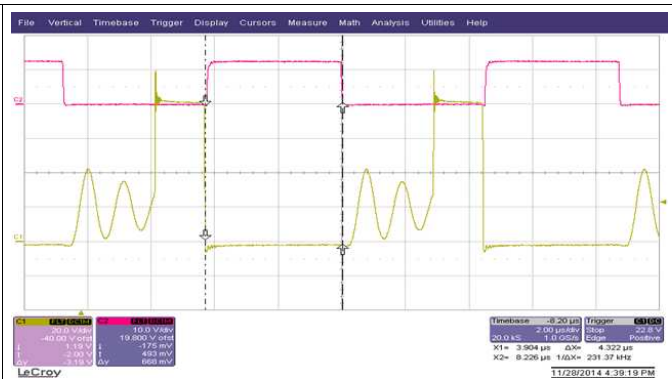
Figure 26. DRV Timing at 115 V AC , 65 W
