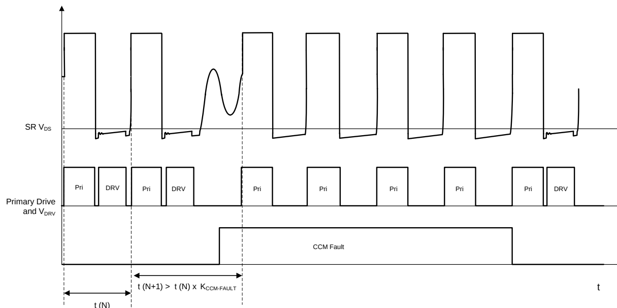
Figure 20. CCM Cycle-Fault Behavior, CCM Operation
