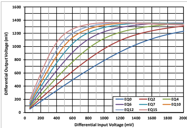
Figure 3. USB TX (UFP) EQ Settings Curves
