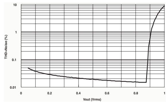
Figure 8. THD + noise vs. output voltage
