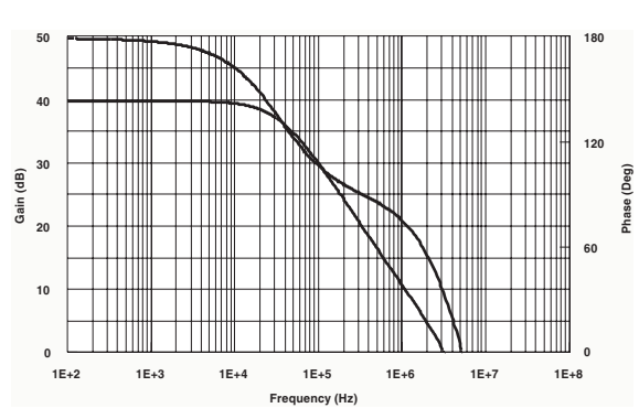
Figure 12. Open loop gain and phase vs. frequency
