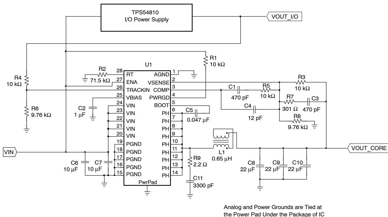
Figure 8. Application Circuit
