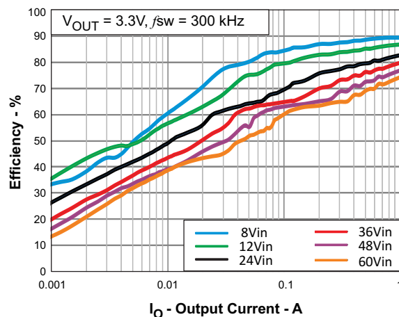
Figure 49. Light Load Efficiency
