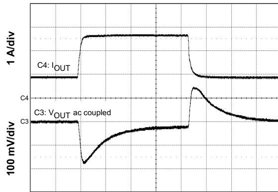
Figure 34. Load Transient
