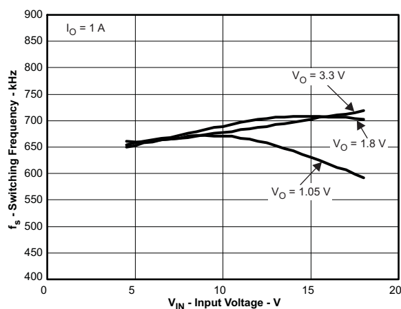
Figure 9. SWITCHING FREQUENCY vs INPUT VOLTAGE
