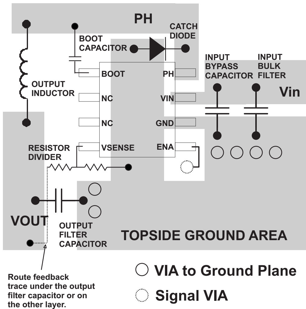
Figure 9. Design Layout
