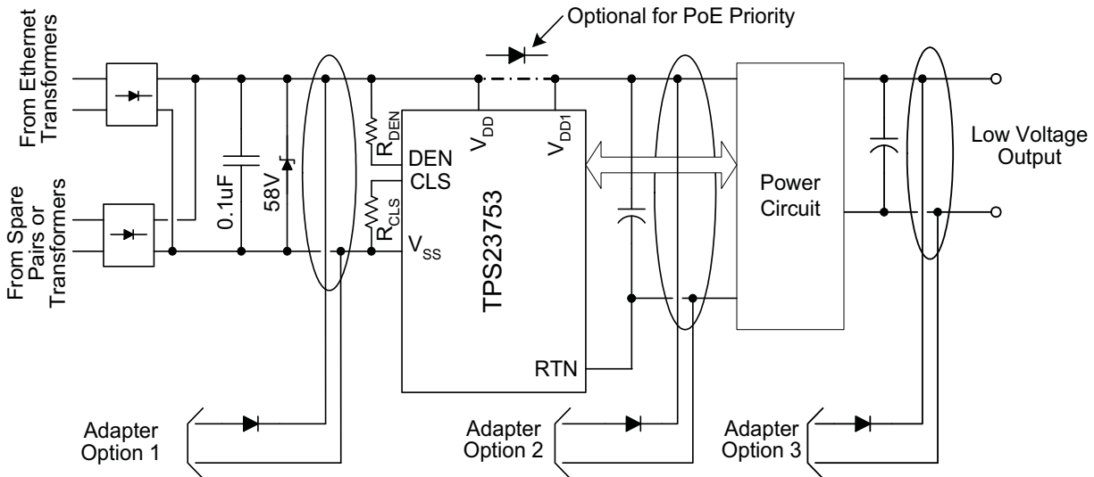
Figure 24. ORing Configurations
