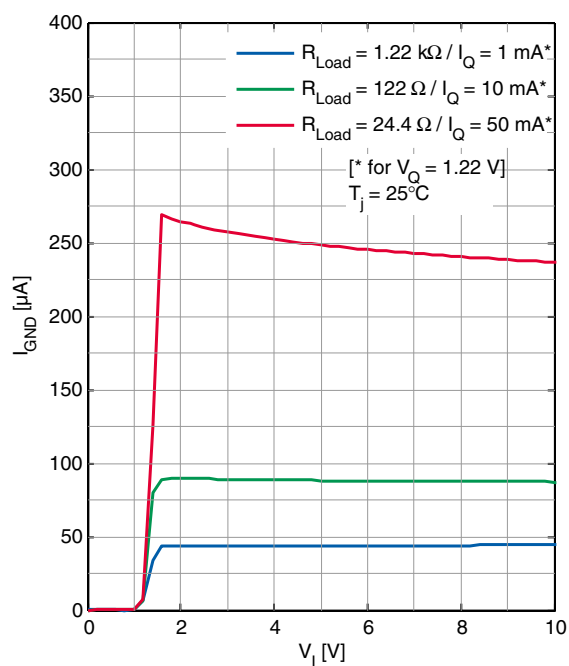
GND Pin Current I_{\text{GND}} versus Input Voltage V_i (TLS203B0EJV)
