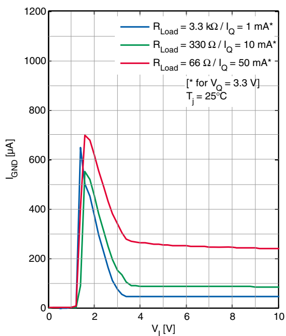
GND Pin Current I_{\text{GND}} versus Input Voltage V_i (TLS203B0EJV33)
