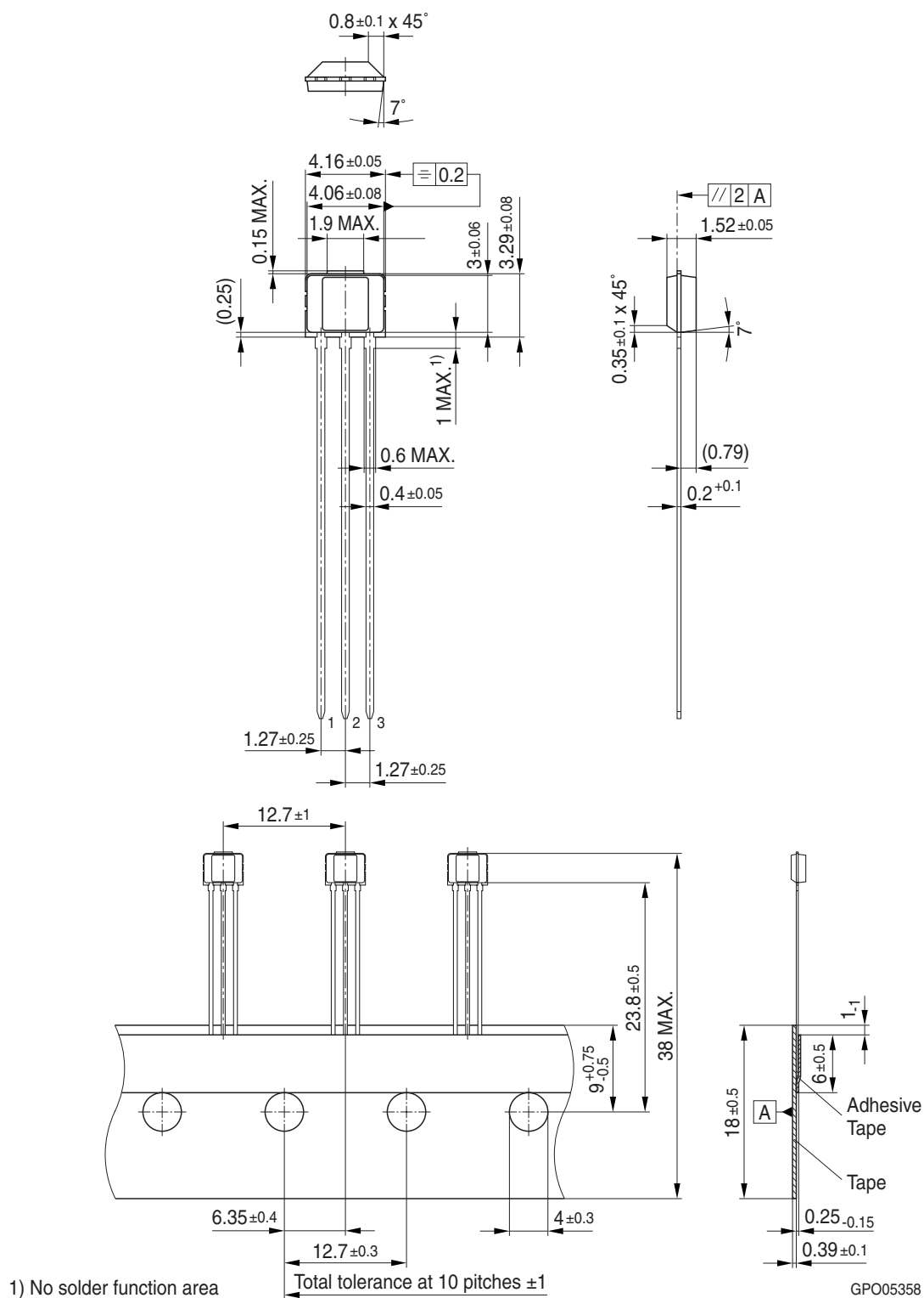
Figure 11 PG-SSO-3-2 Package Outline
