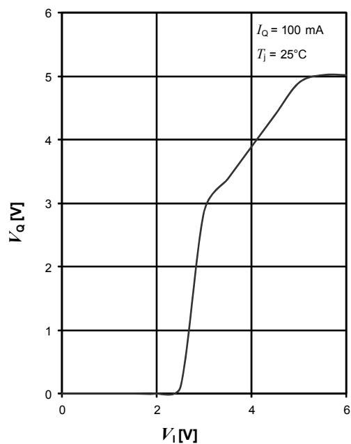
Output Voltage V_O versus Input Voltage V_I (TLF80511TFV50)
