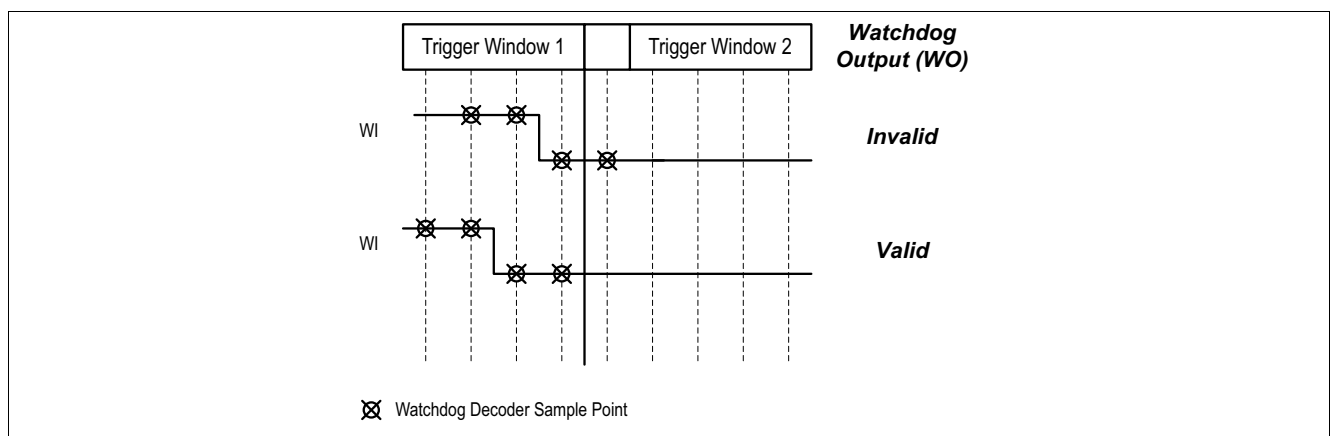
Figure 8 Valid triggering
