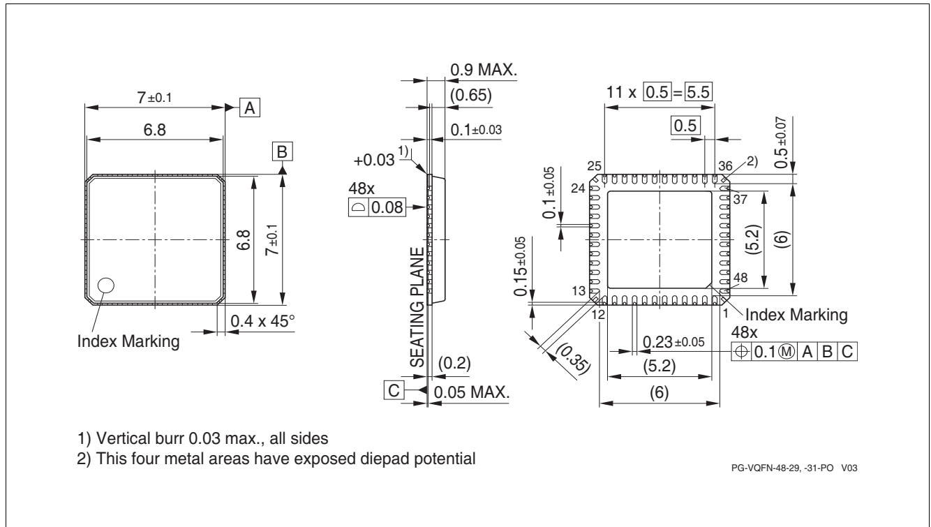
Figure 58 PG-VQFN-48-31
