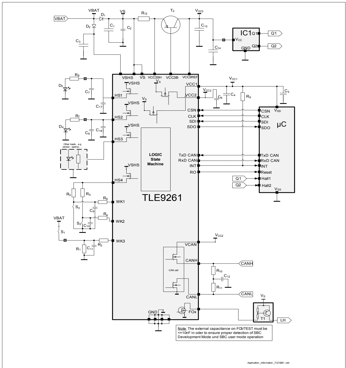
Figure 54 Simplified Application Diagram
