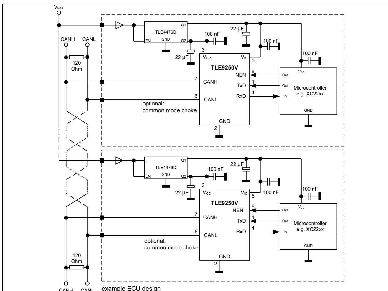
Figure 15 Application circuit
