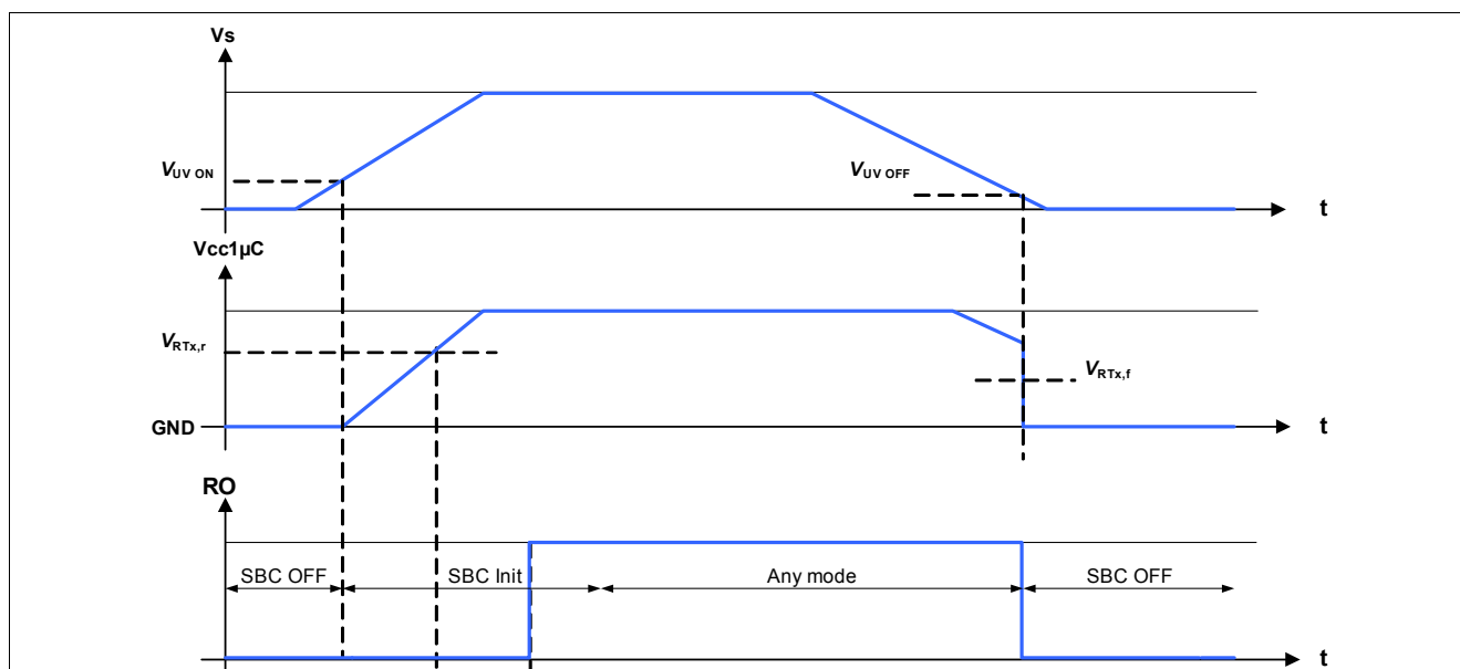
Figure 5 Ramp up / Down of Main Voltage Regulator
