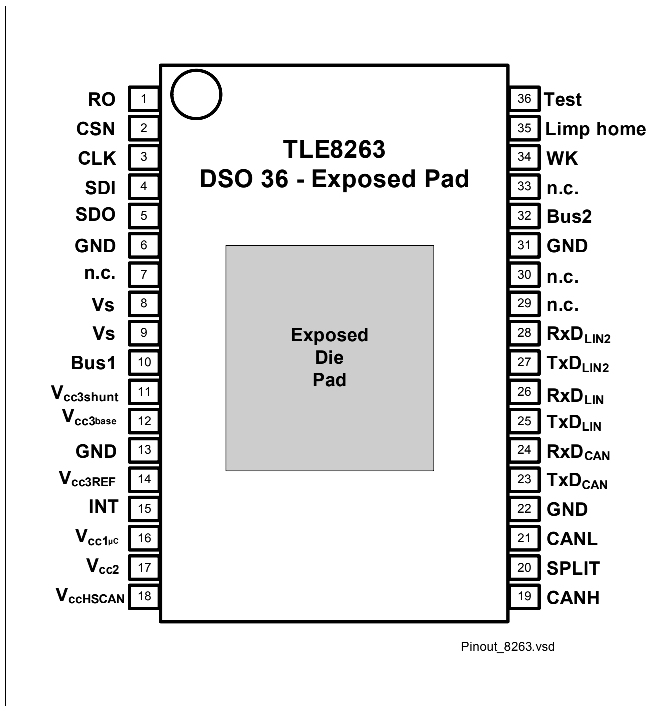
Figure 2 Pin Configuration
