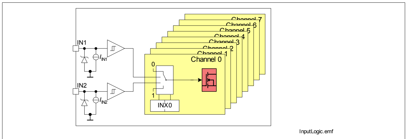
Figure 4 Input Multiplexer
