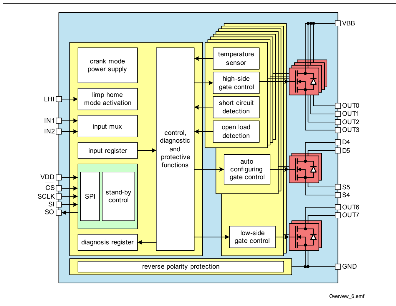
Figure 1 Block Diagram
