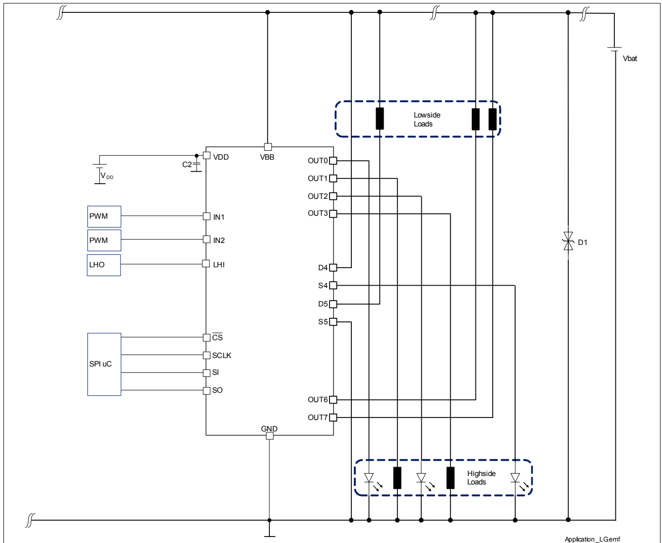
Figure 14 Application Diagram
