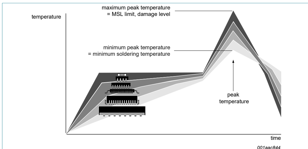
Figure 16. Temperature profiles for large and small components
