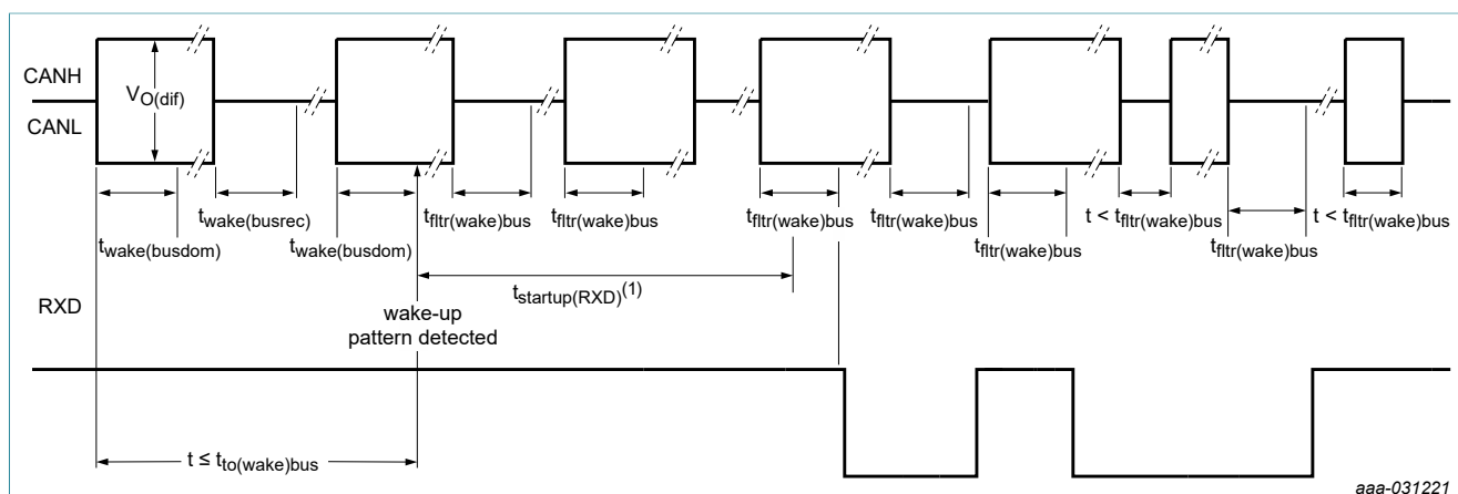
Figure 6. Wake-up timing
