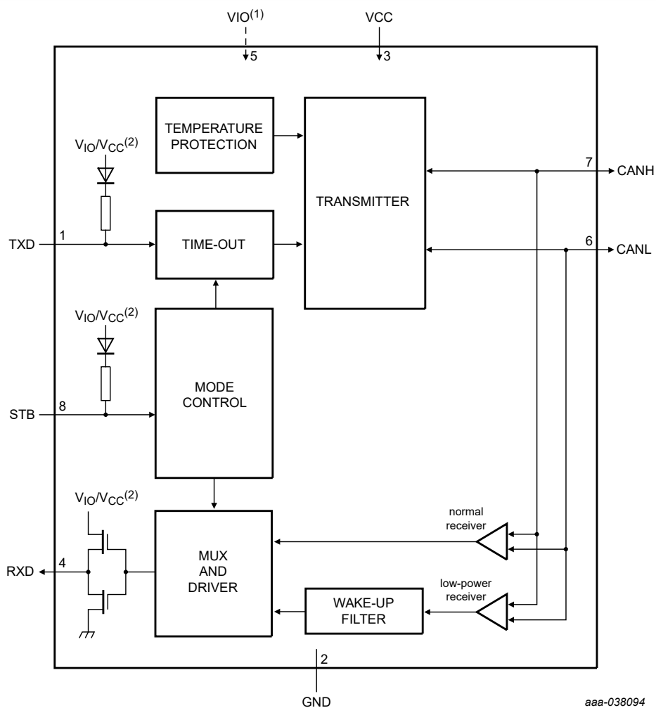
Figure 1. Block diagram
