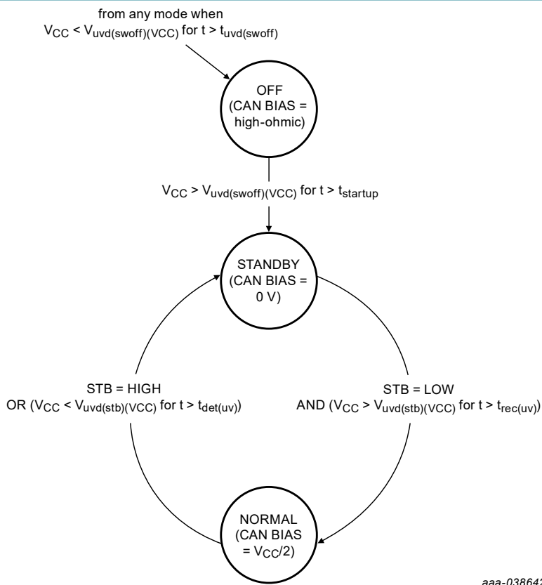
Figure 4. TJR1442B state diagram
