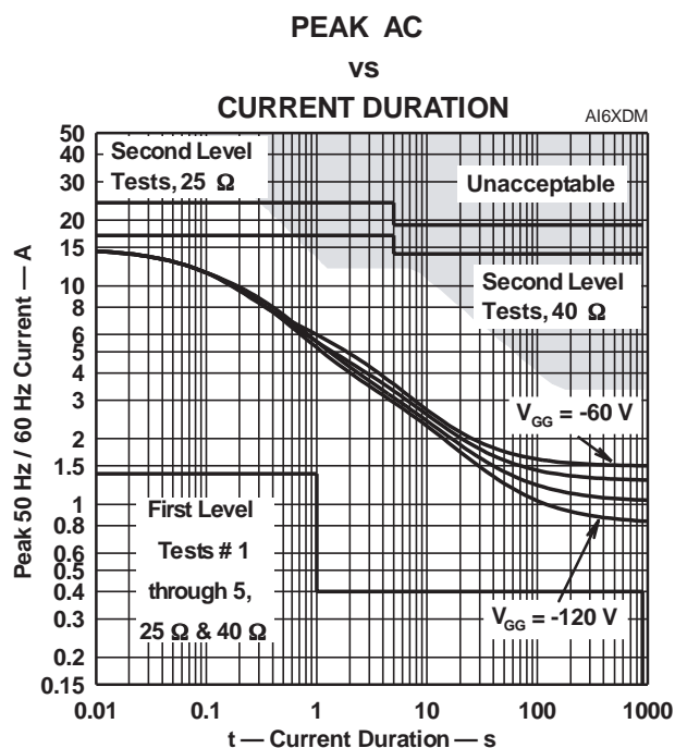
Figure 19. TISP61089B Overlay
