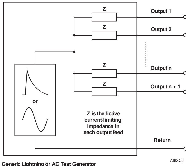
Figure 13. '1089 Test Generators
