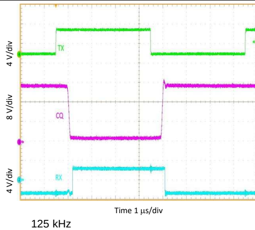
Figure 20. CQ in Communication Mode
