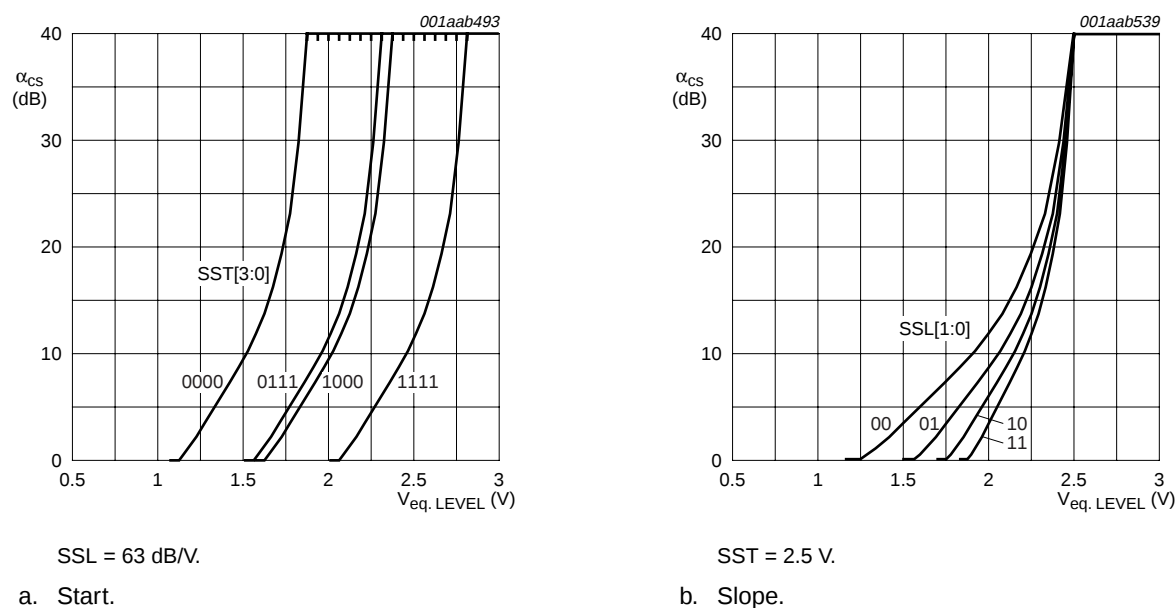
Fig 25. SNC start and slope settings versus equivalent level voltage; SNC detector (level, USN and WAM), USN detector and WAM detector
