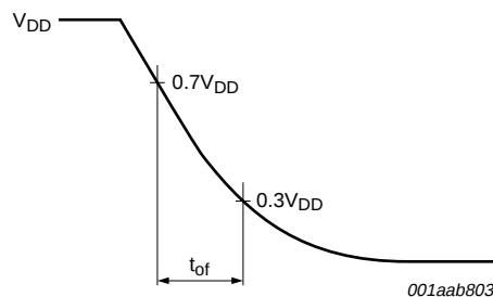
Fig 40. Definition of the fall time of the output signal
