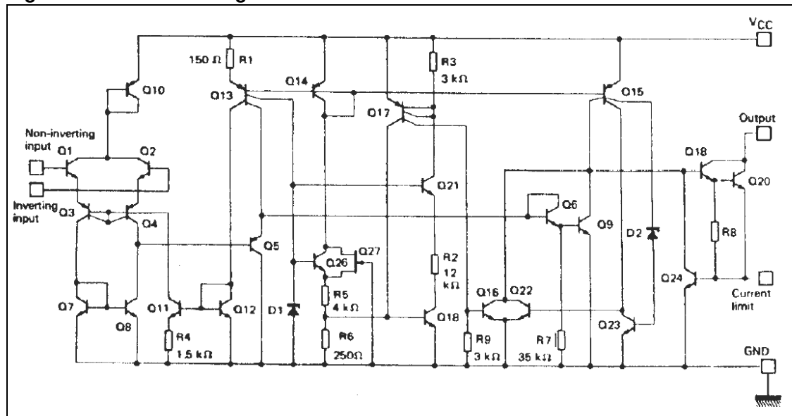
Figure 2. Schematic diagram
