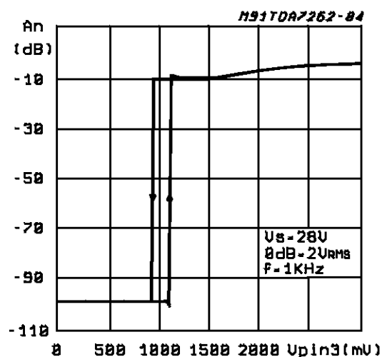
Figure 8: Output Attenuation vs. Vpin 3
