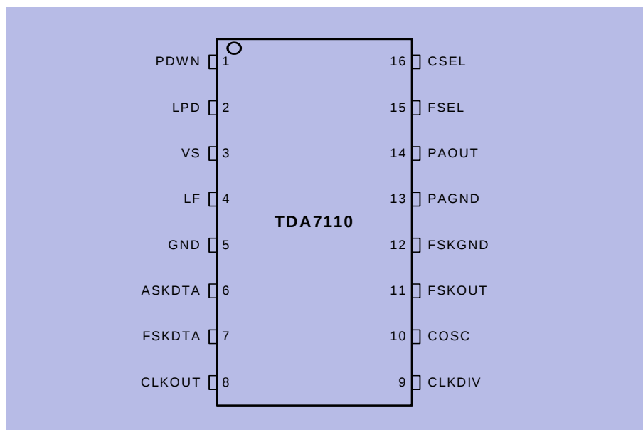
Figure 2-1 IC Pin Configuration
