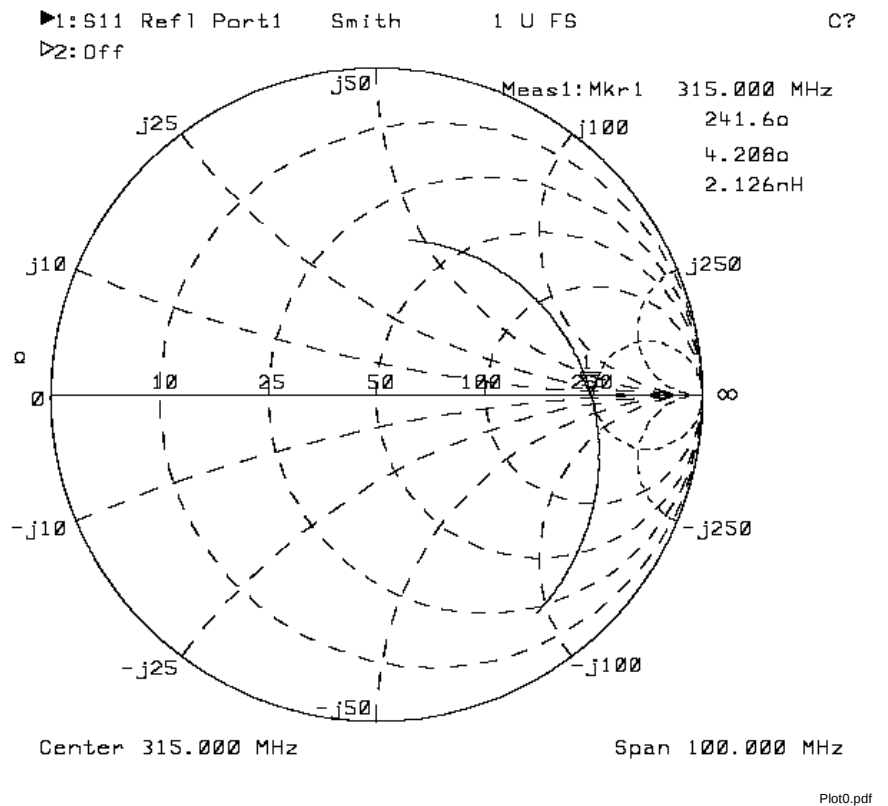
Figure 3-7 Sparam_measured_200M
