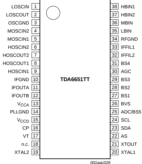
Fig 3. Pin configuration TDA6651TT
