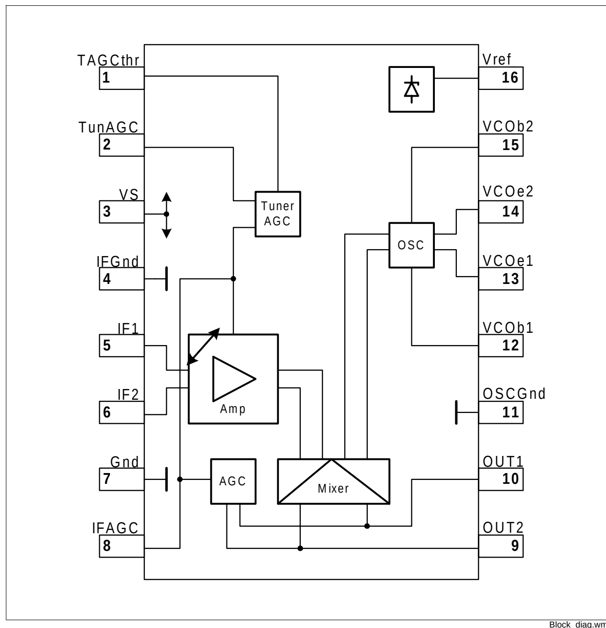
Figure 2-3 Block Diagram
