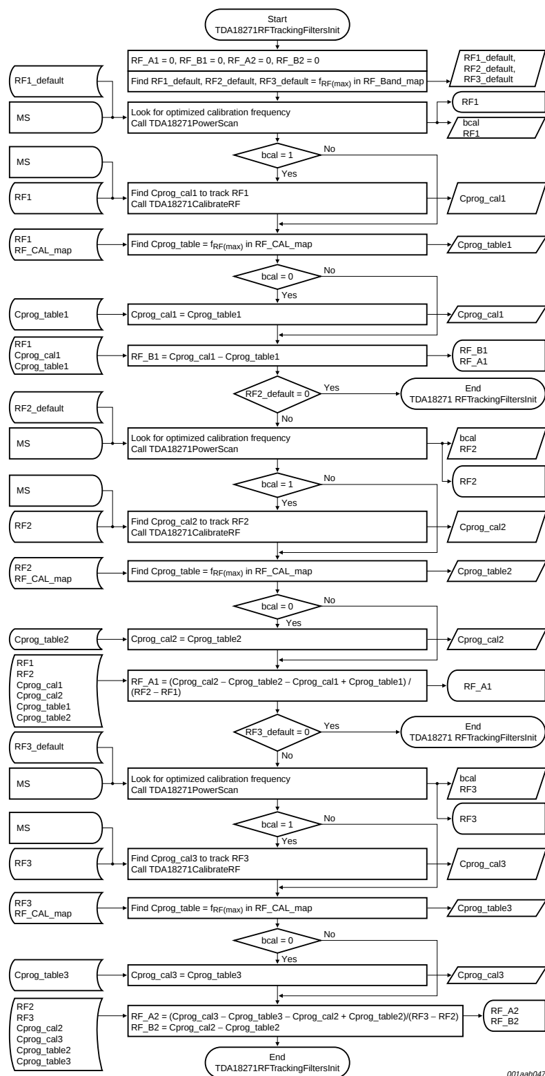
Fig 11. Flowchart TDA18271RFTrackingFiltersInit
