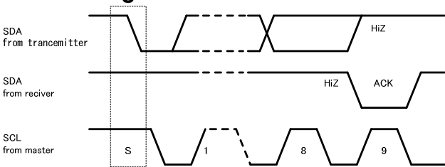
Figure 3 Start/End condition
