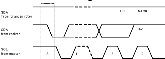
Figure 3 Start/End condition
