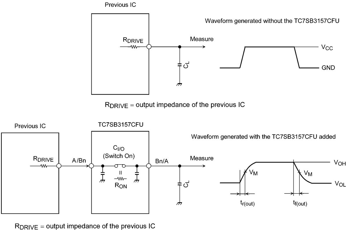
Fig. 11.1 Calculation Circuit
