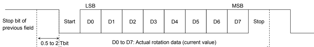
Figure 7.18 DATA1 Field
