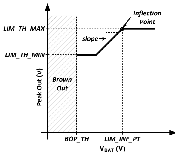
Figure 8-17. Limiter with Inflection Point and Minimum Threshold
