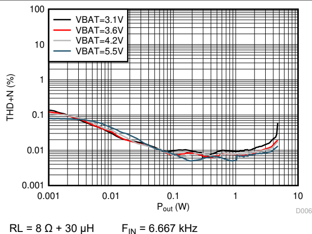
Figure 6-10. THD+N vs Output Power
