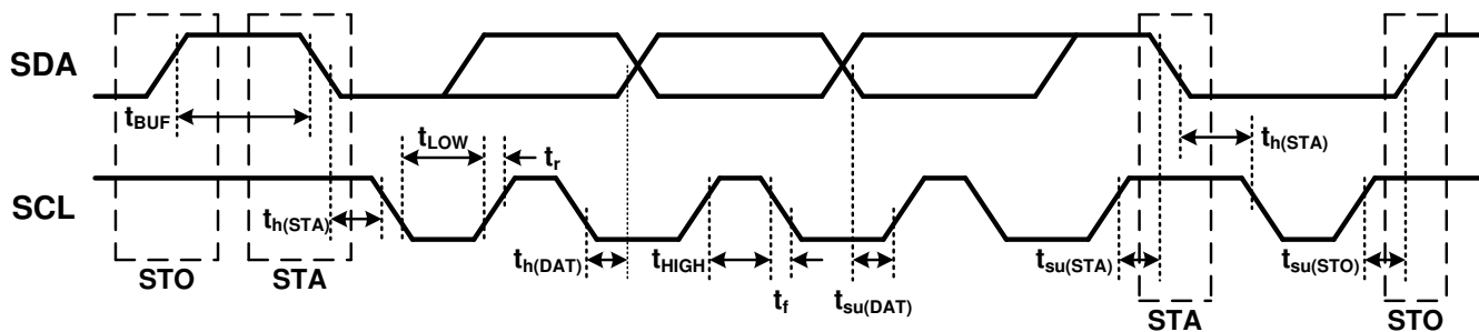
Figure 6-1. I²C Timing Diagram
