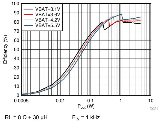
Figure 6-23. Efficiency vs Output Power
