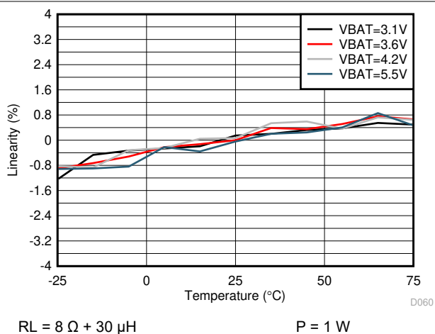
Figure 6-47. V/I-sense Linearity vs Temperature
