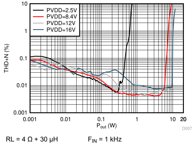
Figure 6-11. THD+N vs Output Power
