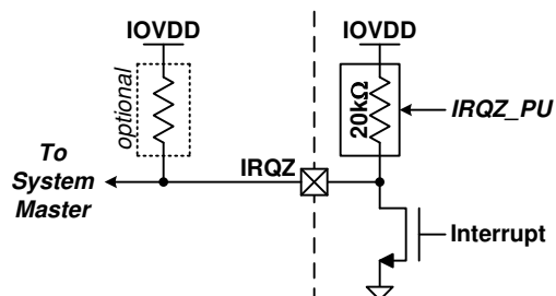
Figure 8-10. IRQZ Pin
