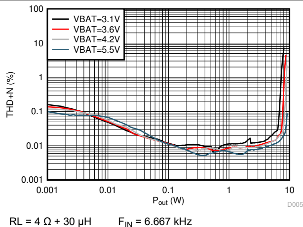
Figure 6-9. THD+N vs Output Power
