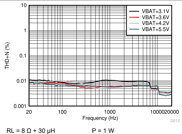
Figure 6-16. THD+N vs Frequency
