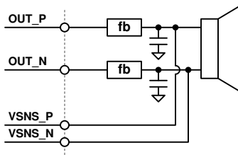
Figure 8-19. V-Sense Connections
