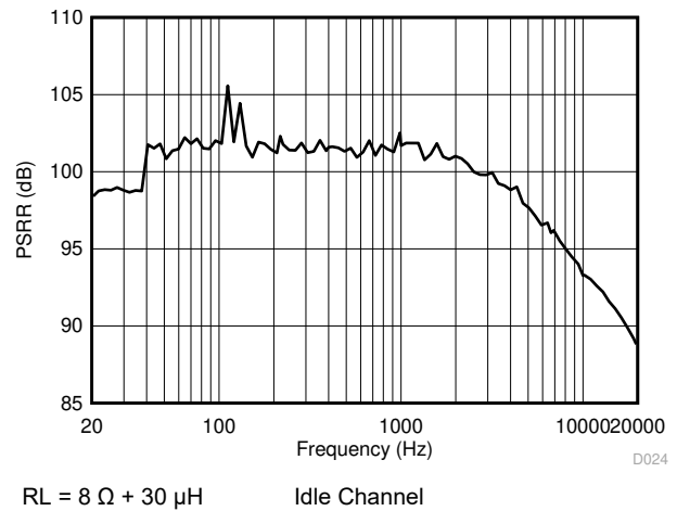
Figure 6-26. AVDD PSRR vs Frequency
