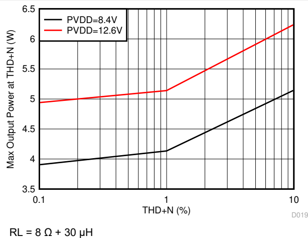
Figure 6-21. Max Output Power vs THD+N
