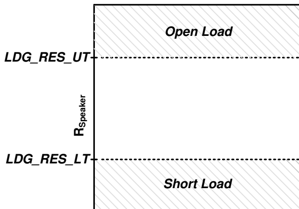
Figure 8-20. Load Diagnostics
