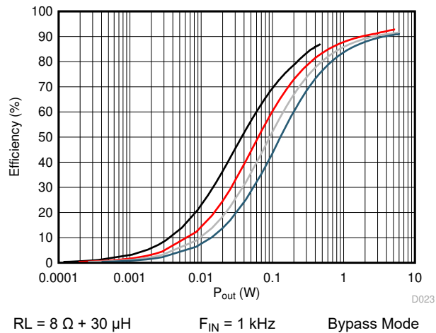
Figure 6-25. Efficiency vs Output Power
