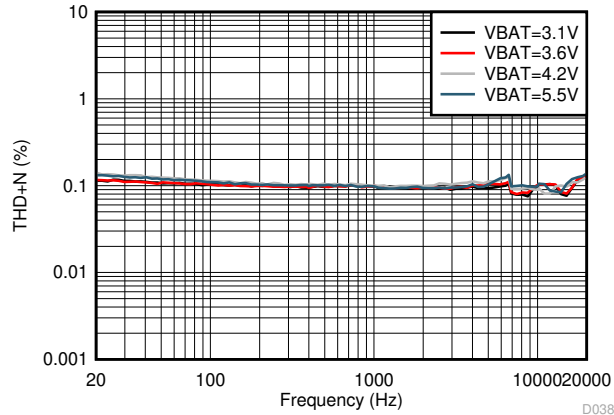
Figure 6-35. I-sense THD+N vs Frequency
