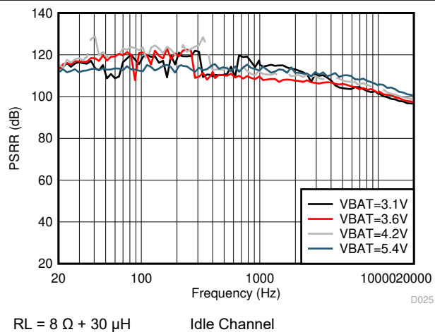
Figure 6-27. VBAT PSRR vs Frequency
