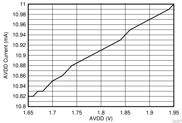
Figure 6-29. AVDD Idle Current vs AVDD
