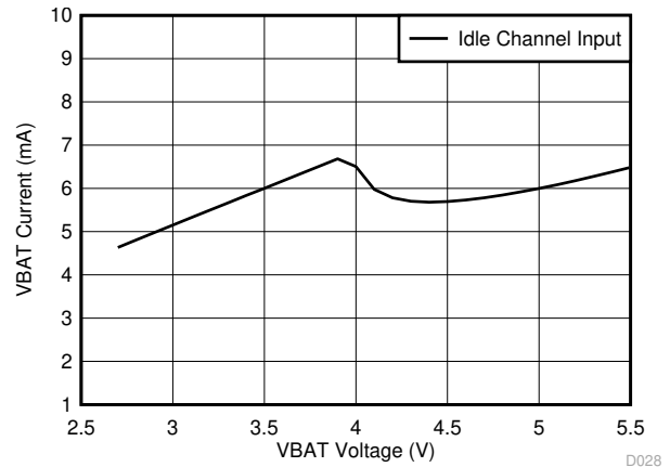
Figure 6-30. VBAT Idle Current vs VBAT
