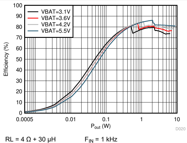
Figure 6-22. Efficiency vs Output Power
