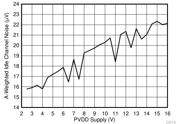
Figure 6-18. Idle Channel Noise (A-Weighted) vs PVDD
