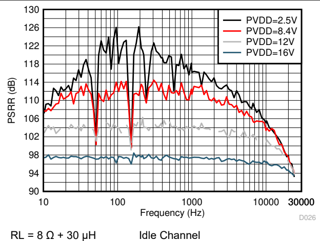
Figure 6-28. PVDD PSRR vs Frequency
