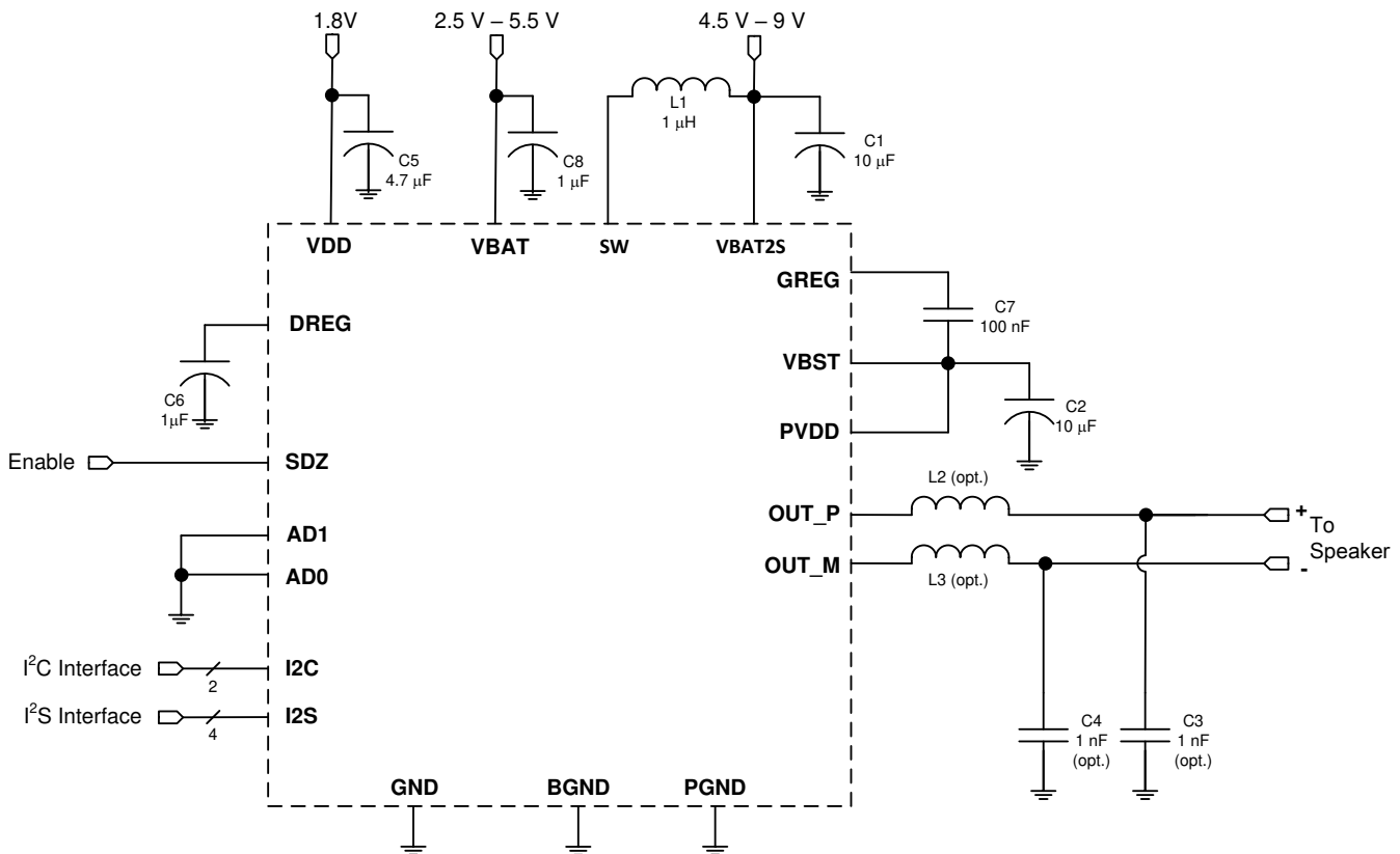
Figure 9-1. Typical Application - Digital Audio Input
