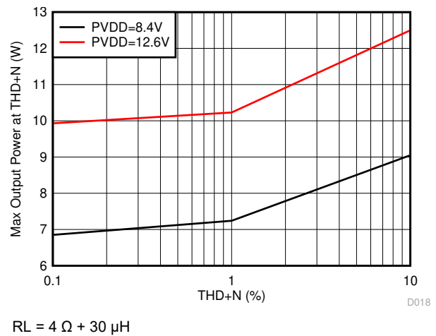
Figure 6-20. Max Output Power vs THD+N
