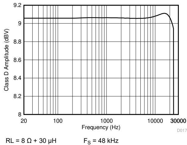
Figure 6-19. Amplitude vs Frequency
