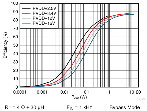
Figure 6-24. Efficiency vs Output Power
