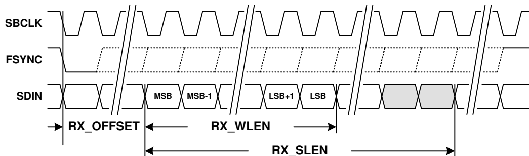
Figure 8-12. TDM RX Time Slot with Left Justification
