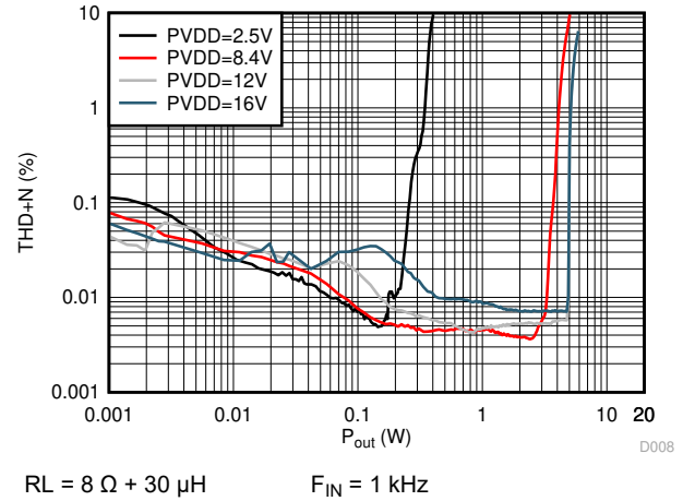
Figure 6-12. THD+N vs Output Power
