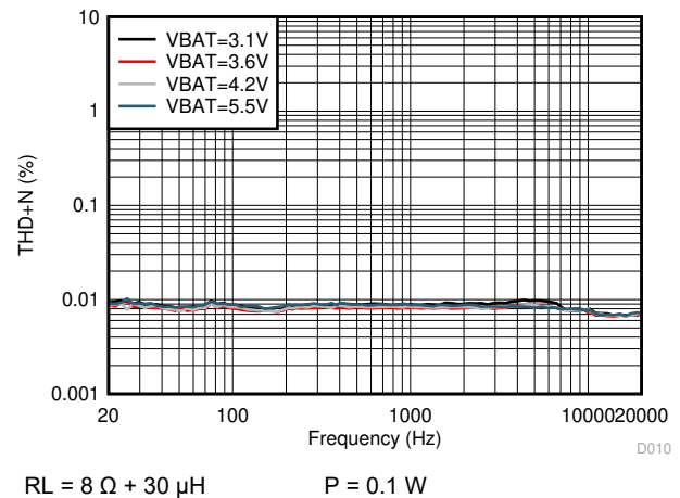
Figure 6-14. THD+N vs Frequency
