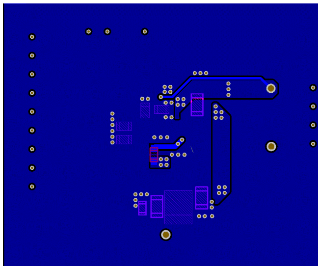
Figure 11-8. QFN Package Bottom Layer
