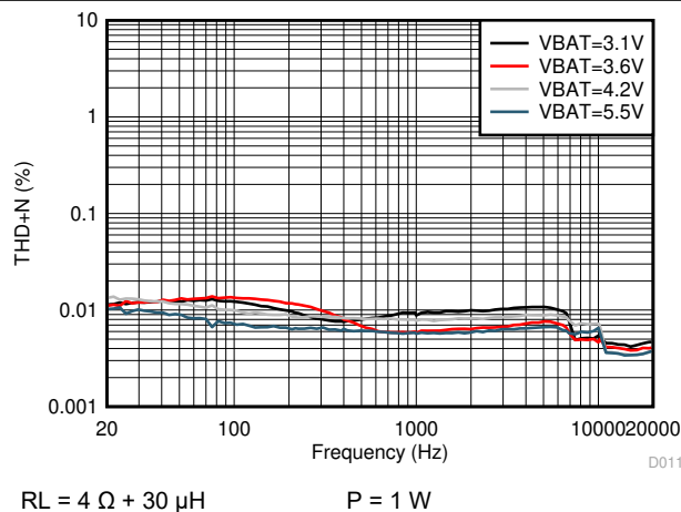
Figure 6-15. THD+N vs Frequency
