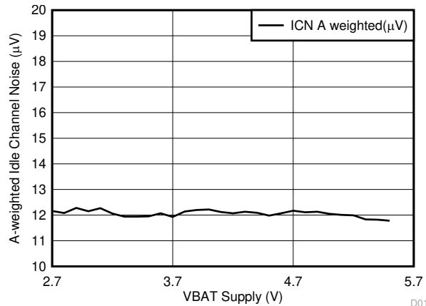
Figure 6-17. Idle Channel Noise (A-Weighted) vs VBAT
