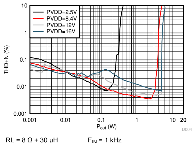
Figure 6-8. THD+N vs Output Power
