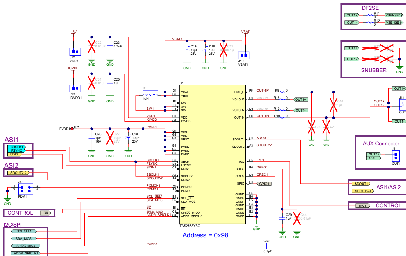
Figure 7-1. TAS2563 Circuit
