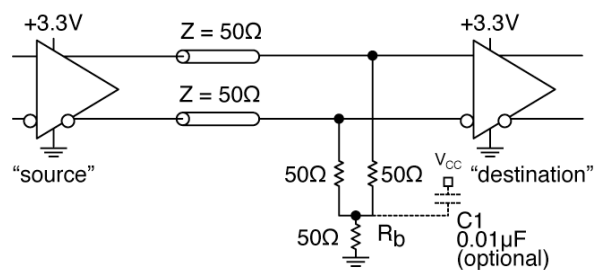
Figure 2. Three-Resistor "Y-Termination"
