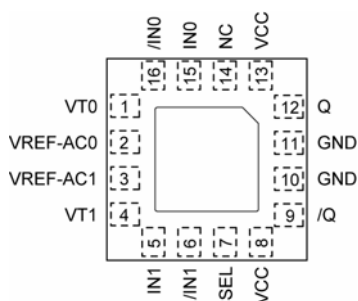
16-Pin MLF ® (MLF-16)
