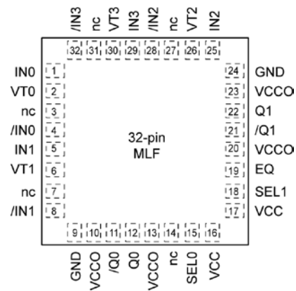
32-Pin QFN
