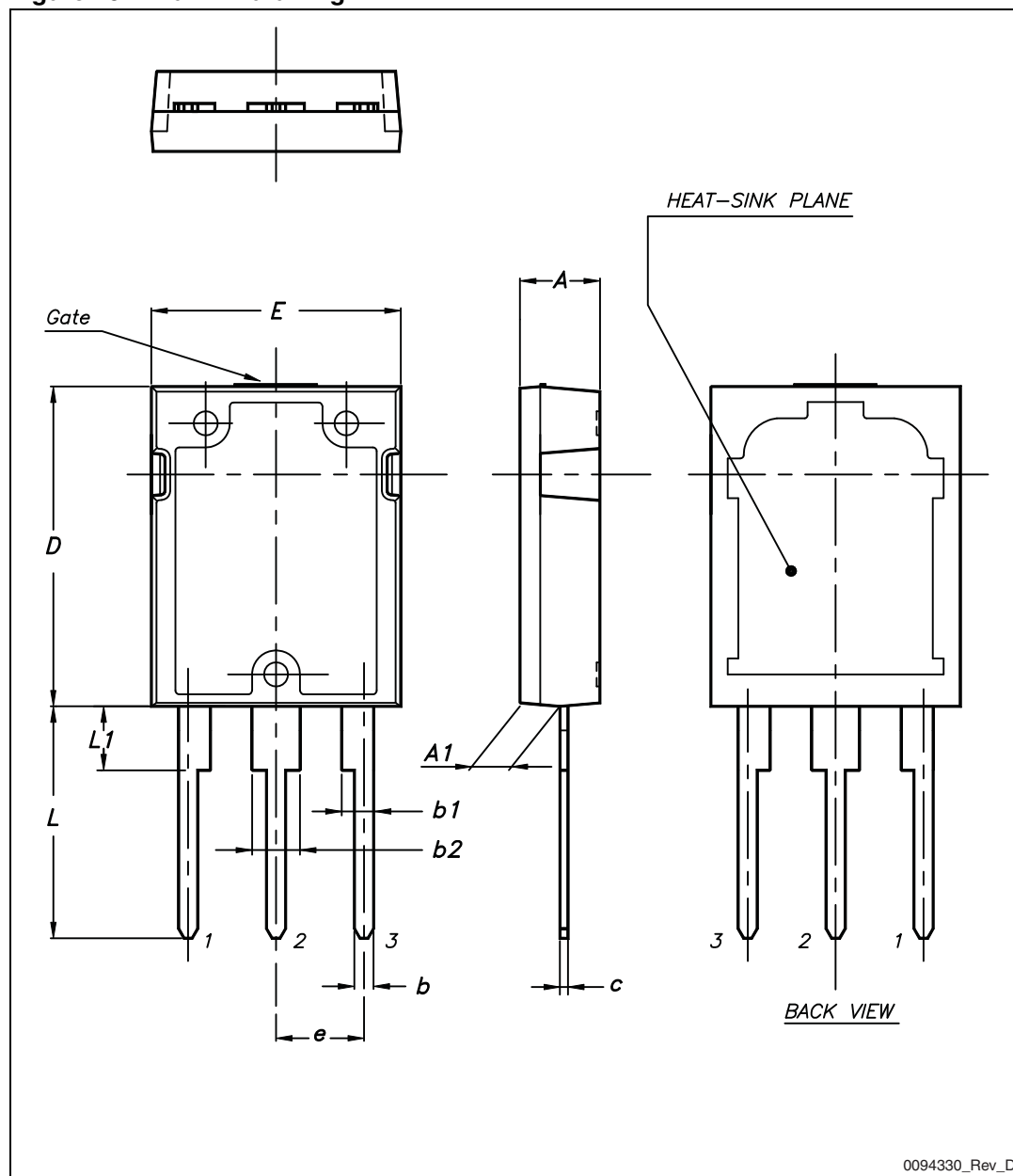
Figure 20. Max247 drawing
