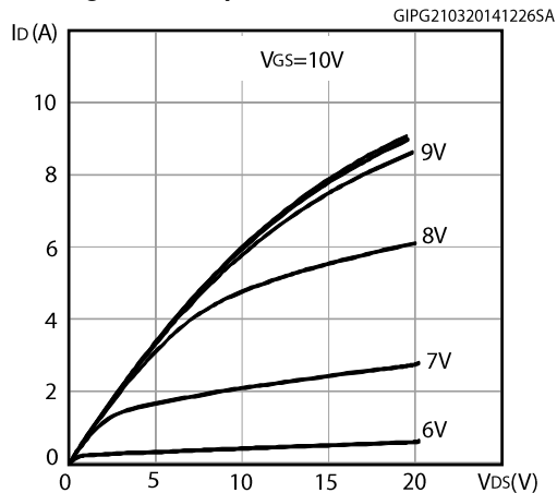
Figure 6: Output characteristics
