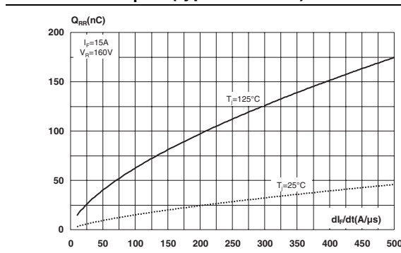
Figure 7. Reverse recovery charges versus dl_F/dt (typical values)
