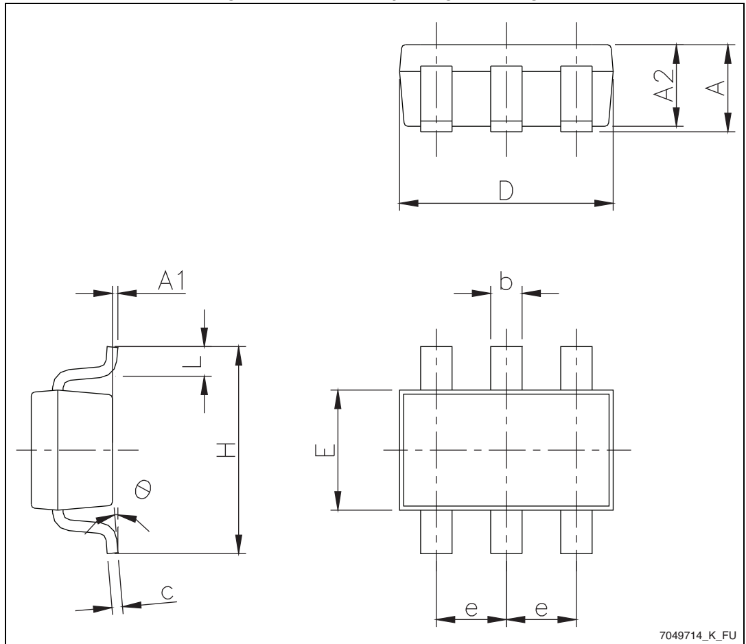
Figure 19. SOT23-6L package drawing
