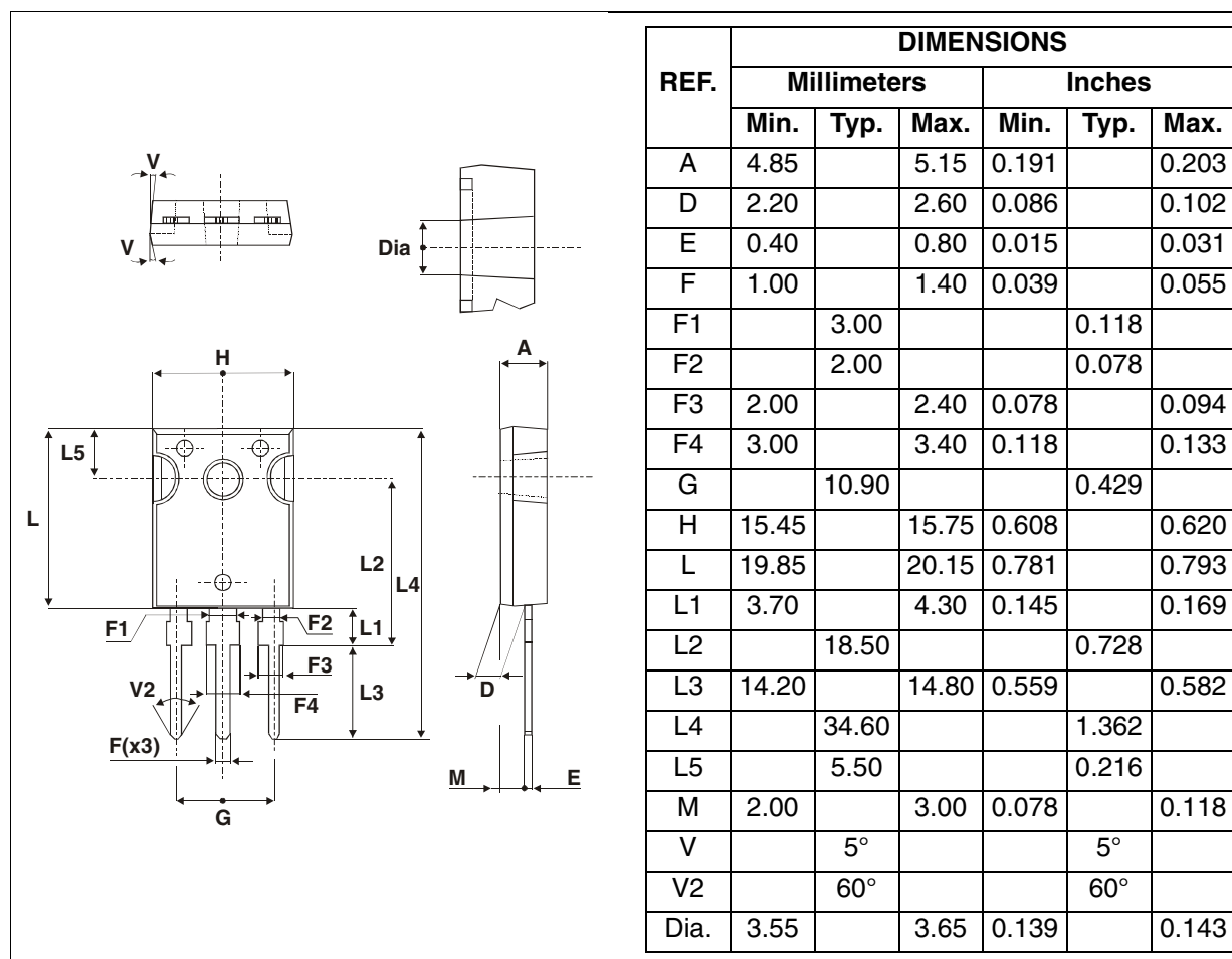
Figure 11: TO-247 Package Mechanical Data
