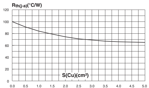
Figure 14: Thermal resistance junction to ambient versus copper surface under each lead (Epoxy printed circuit board FR4, copper thickness: 35μm) (SMB)
