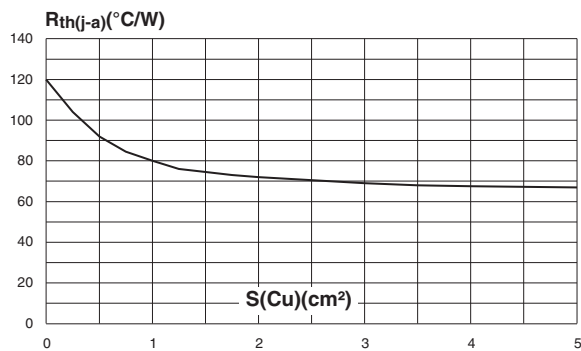
Figure 13: Thermal resistance junction to ambient versus copper surface under each lead (Epoxy printed circuit board FR4, copper thickness: 35μm) (SMA)
