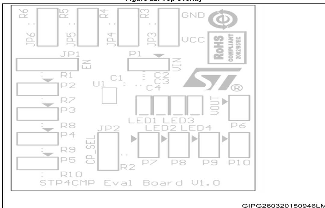
Figure 11: Top overlay
